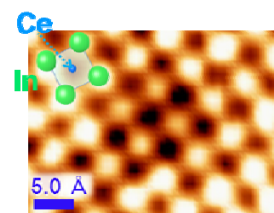
Fig.1. Topographic image of Ce 0.98 Nd 0.02 CoIn 5 thin film at 0.3 K .
