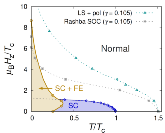
Fig. 1. Calculated phase diagram of dilute superconducting \text{SrTiO}_3 with polar lattice instability. Ferroelectric superconducting phase (SC+FE) is stabilized even though the normal state is paraelectric.
