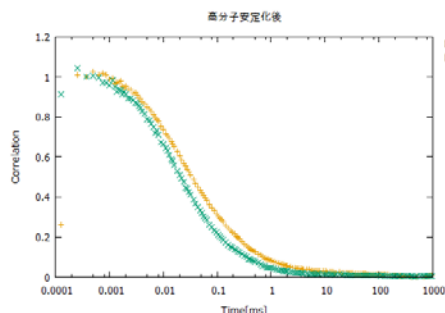
Fig.3 Autocorrelation function.
