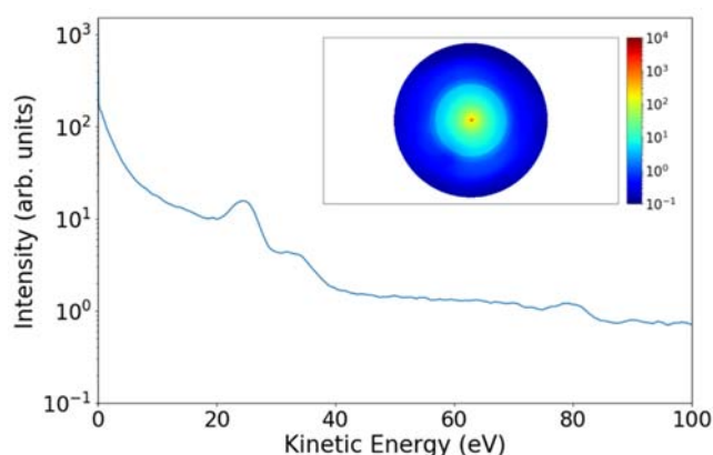
Fig. 1. Electron kinetic energy spectrum and 2-D projection image of electron momentum distribution (inset) measured after ionization of \text{Xe}_{200} cluster with FEL pulses (peak fluence : 6 \times 10^{-3} \mu\text{J}/\mu\text{m}^2 ).
