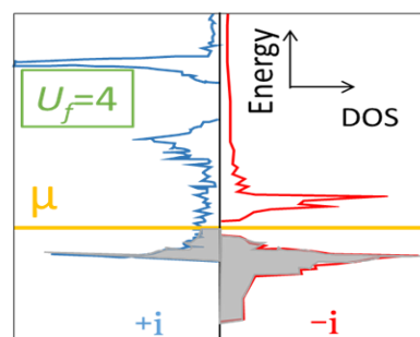
Fig.2 DOS about half-metal ferromagnetic phase.
