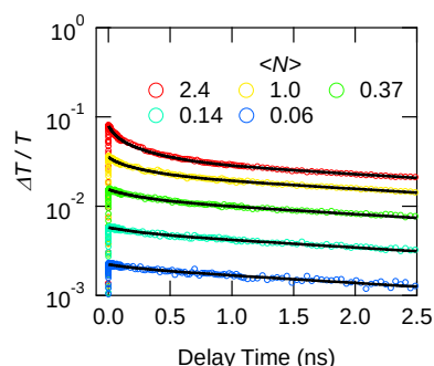
Fig. 1. TA dynamics of untreated NCs. The solid curves are the fitting results. The average number of absorbed photons is denoted by \langle N \rangle .
