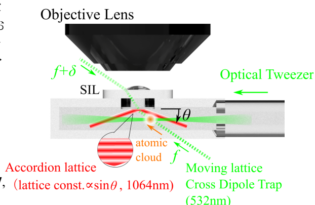
Fig. 1 Schematics of Quantum Gas Microscope: 2D single atom layer just below the SIL is prepared by moving lattice and accordion lattice.
